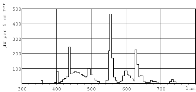
LDPB_TL-D8G_865-Spectral power distribution B/W
